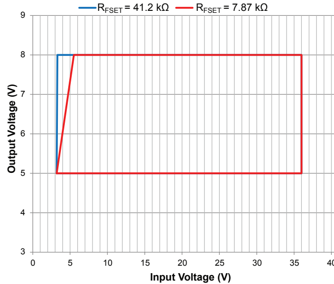
Figure 18: Recommended Operating Range, I_{OUT} = 1\text{ A}
