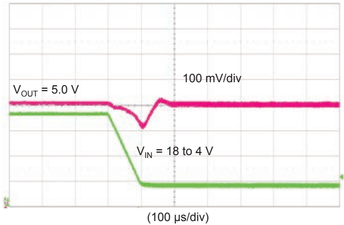
V IN Transient Response: 18 to 4 V at 0.5 A Load for 5 V OUT , 2 MHz design example
