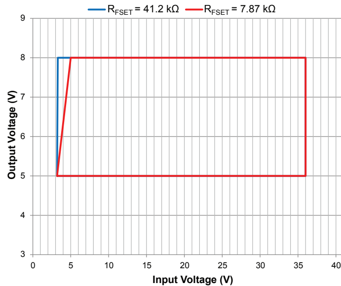
Figure 19: Recommended Operating Range, I_{OUT} = 0.5\text{ A}
