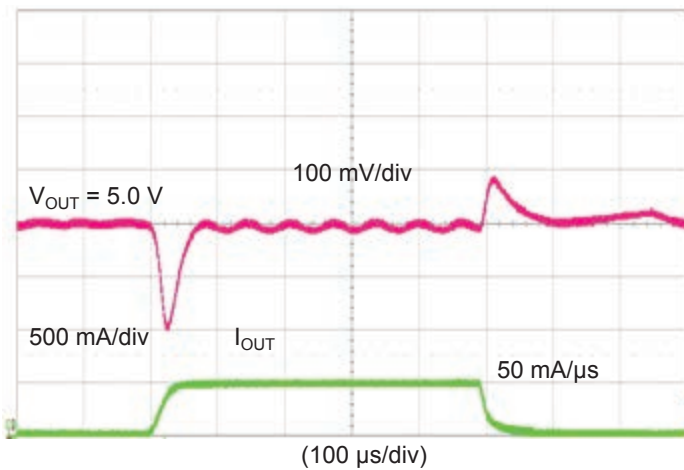
Transient Response 0 to 0.5 A Load Step at V IN = 12 V for 5 V OUT , 2 MHz design example
